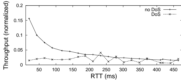
Figure 7: RTT-based filtering
