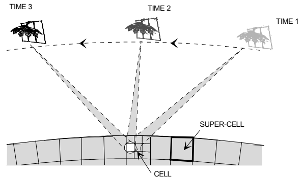
Figure 5. Beam Steering
