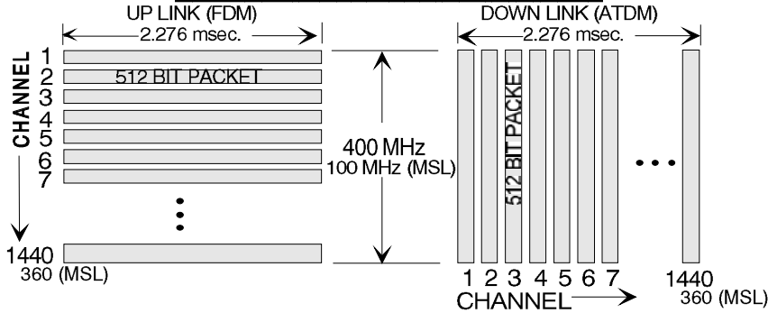
Figure 7. Standard & Mobile Terminal Multiple Access
