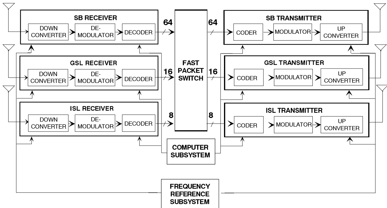
Figure 9. Communications Payload
